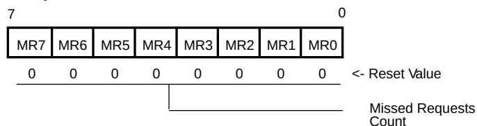
Figure 48. Refresh Register 1
