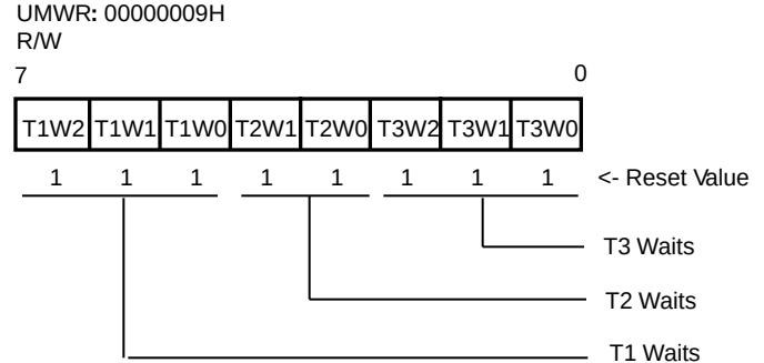
Figure 41. Upper Memory Waits Register
