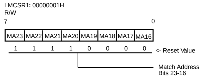
Figure 33. Lower Memory Chip Select Register 1
