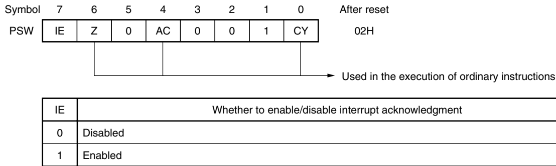
Figure 10-5. Program Status Word (PSW) Configuration
