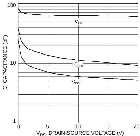
Fig. 9 Typical Capacitance
